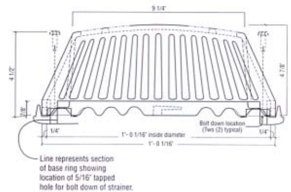
Strainer Elevation
