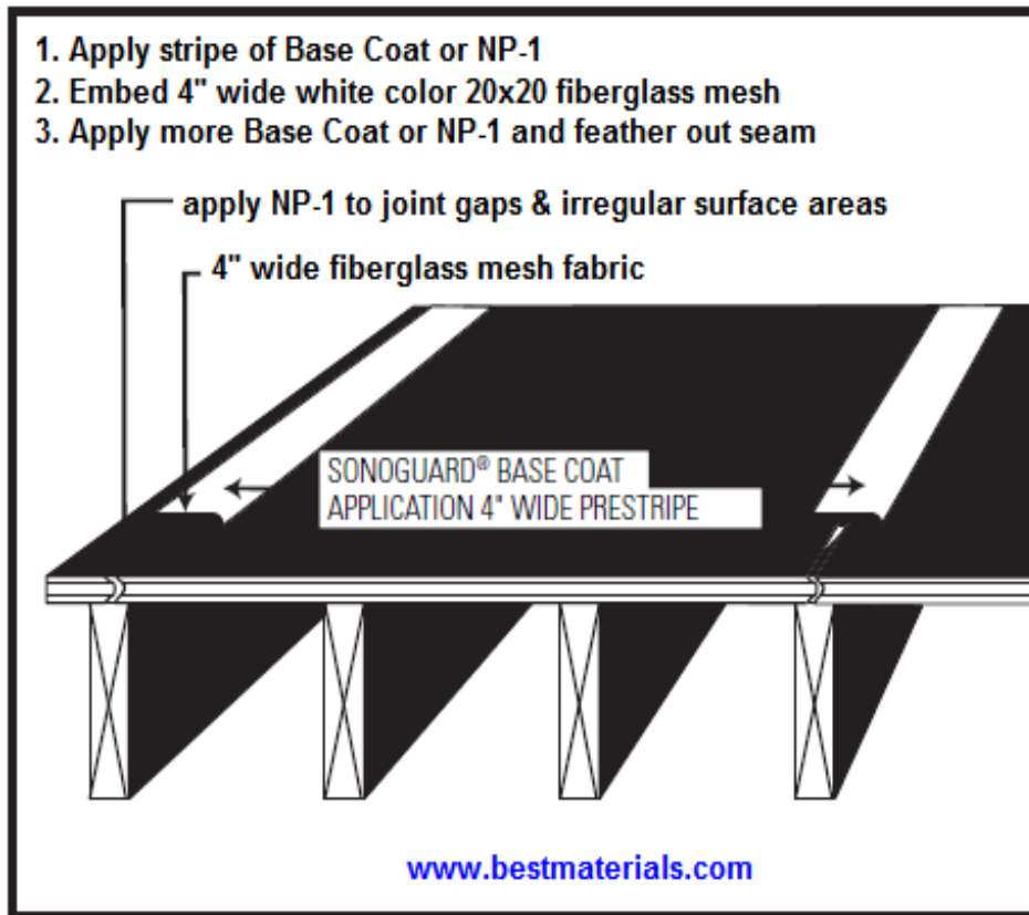
Plywood Application (Seam Detail)
