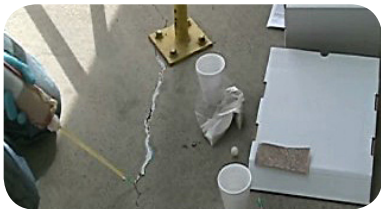
STEP 1: Gravity Feed SlabWeld into Crack
