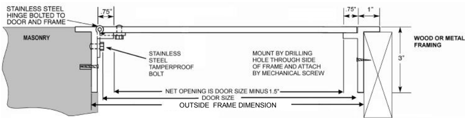
SINGLE DOOR
