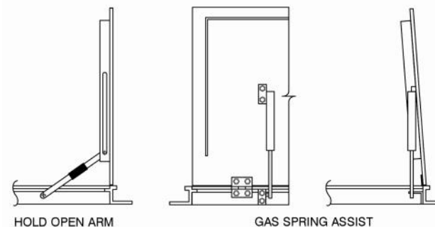
Single Door Construction Shown Above— See Page 2 for Double Door Illustration & Top Views
