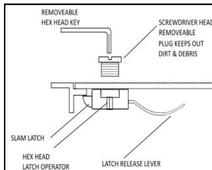
LATCH DETAIL
