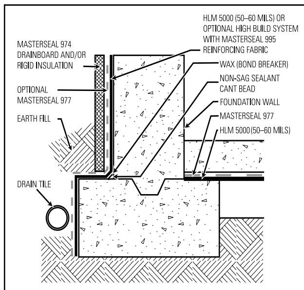
Waterproofing Foundation Walls
