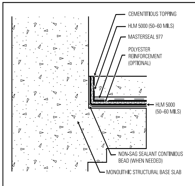
Inside Corner Detail (Static)
