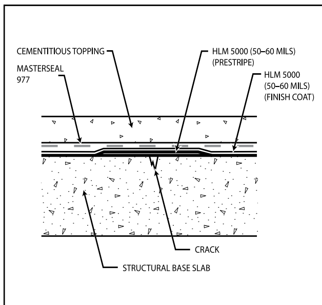
Static Crack/Prestripe Detail
