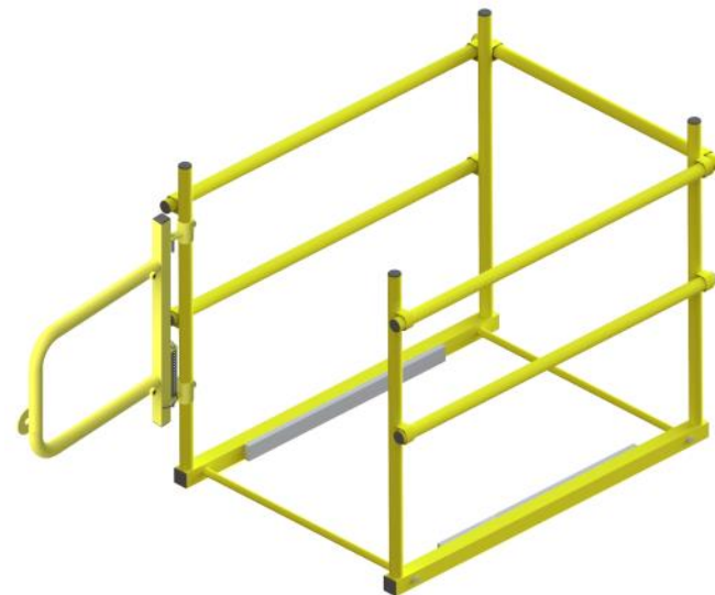
Gate on SHWC 3036 Safety Railing
