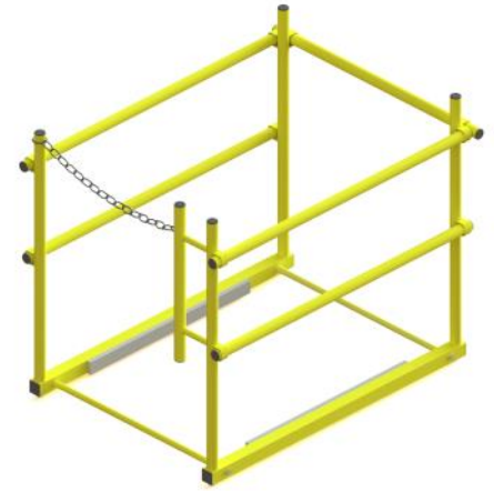
SHWC3636 SHOWN WITH STANDARD GRAB BAR (Standard with 36" and Greater Models)
