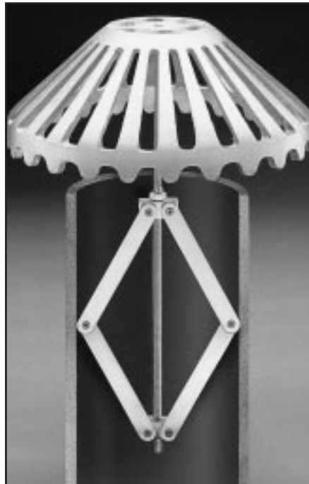
SCISSORS EXPAND TIGHT TO INSIDE OF DRAIN
