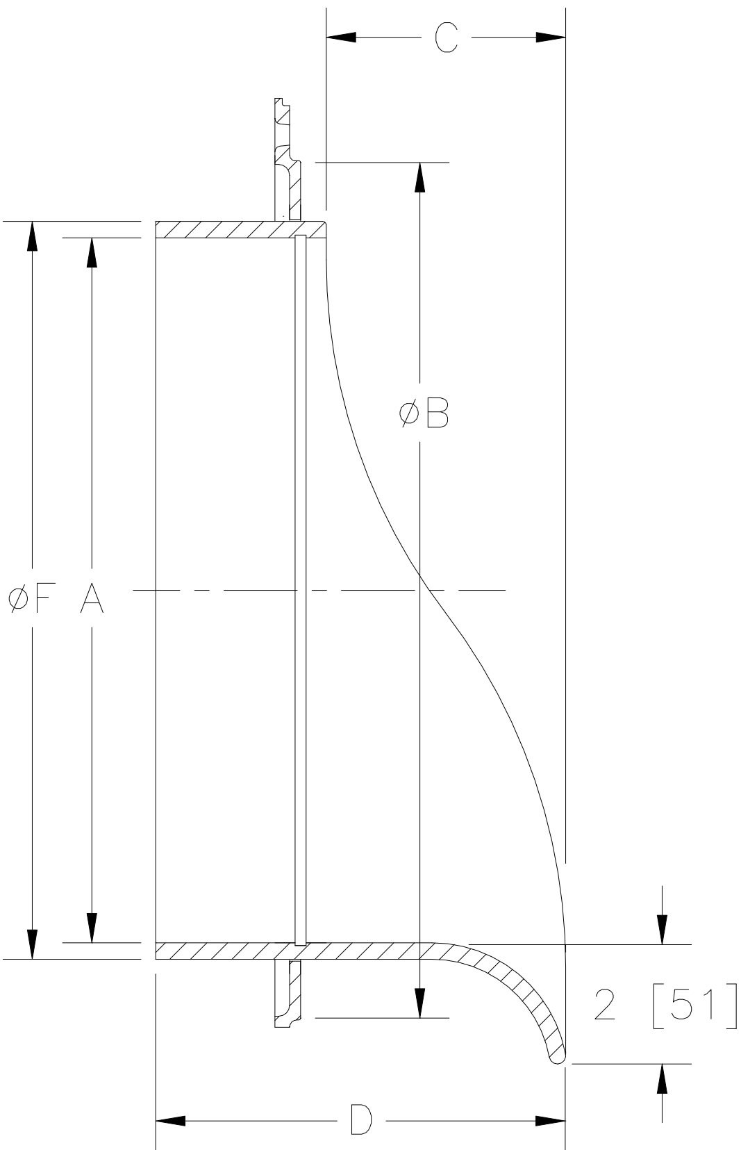
NO-HUB
