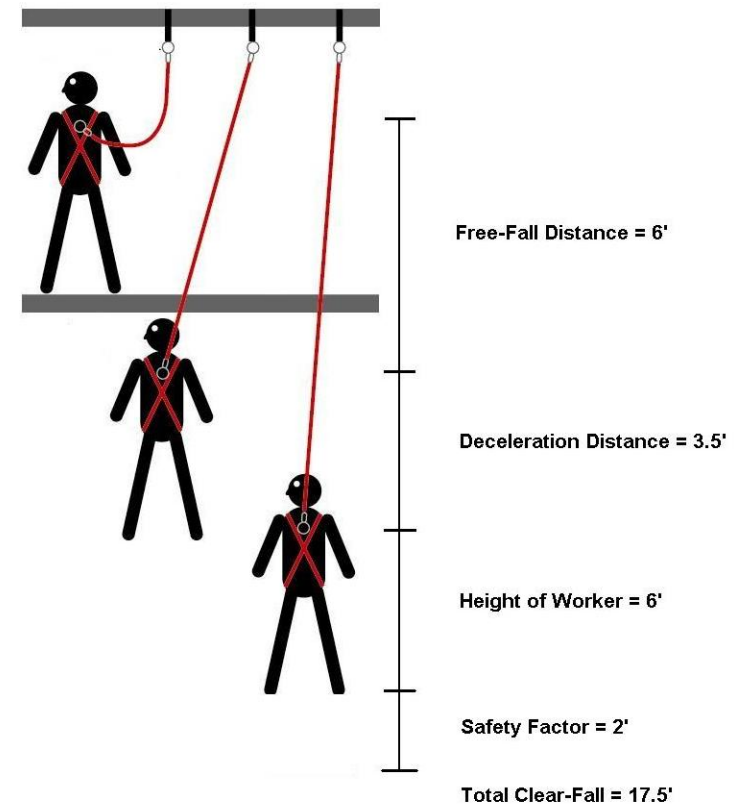
Figure 2.1: Clear-Fall Diagram
